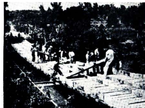
South Vietnamese workers rebuild suspension bridge.
